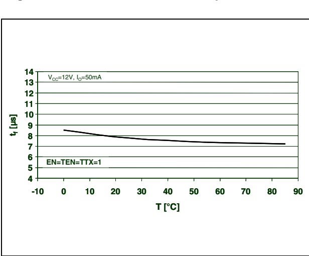
Figure 24. Tone fall time vs. temperature
