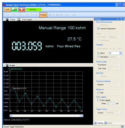
Figure 2. Example of the U2741A KMM Graphical User Interface
