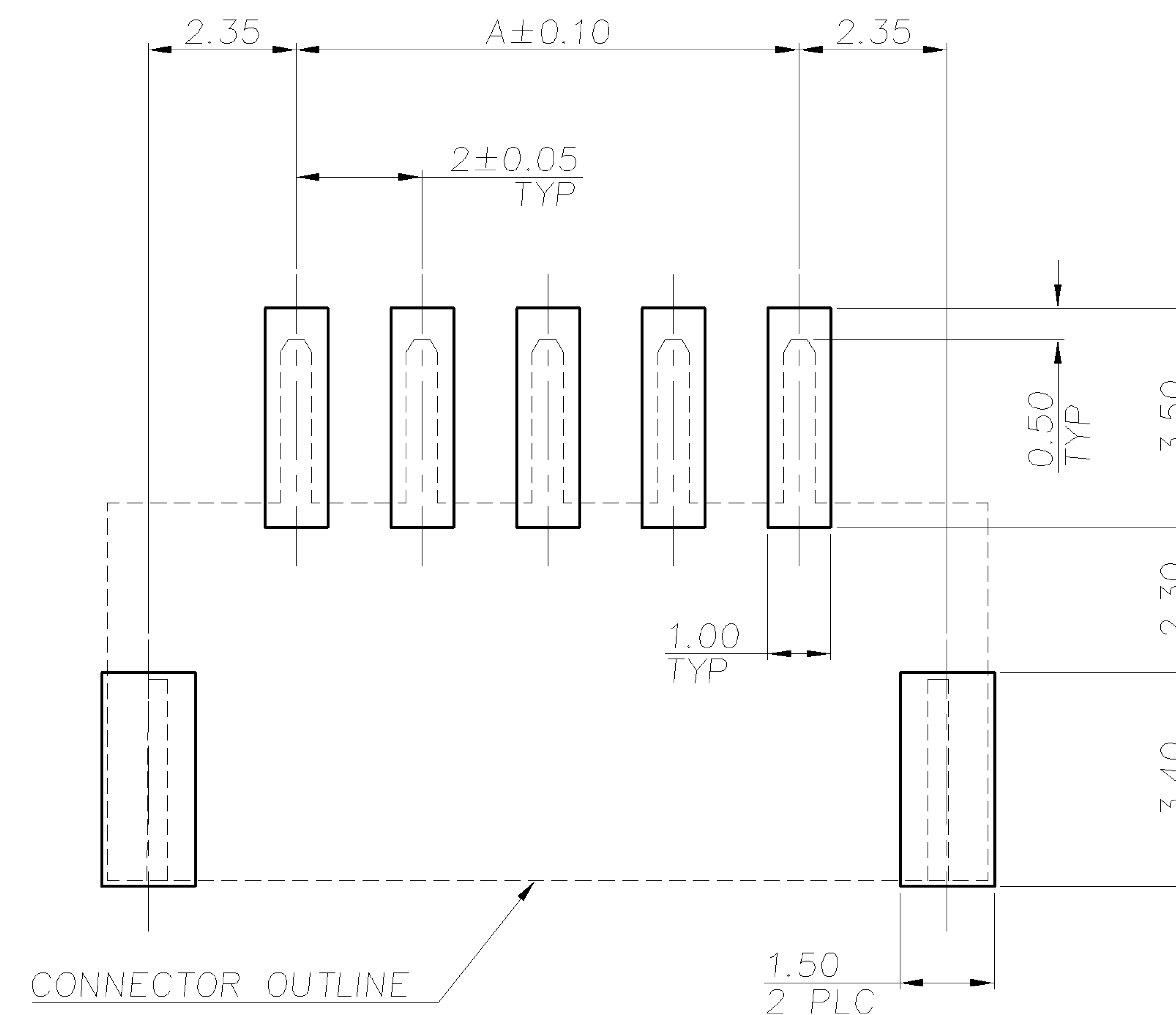
RECOMMENDED PCB LAYOUT
