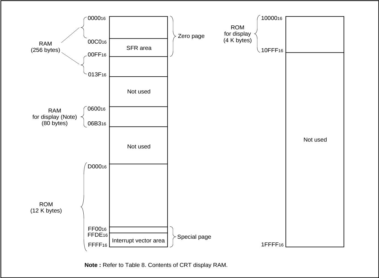
Fig. 2. Memory map
