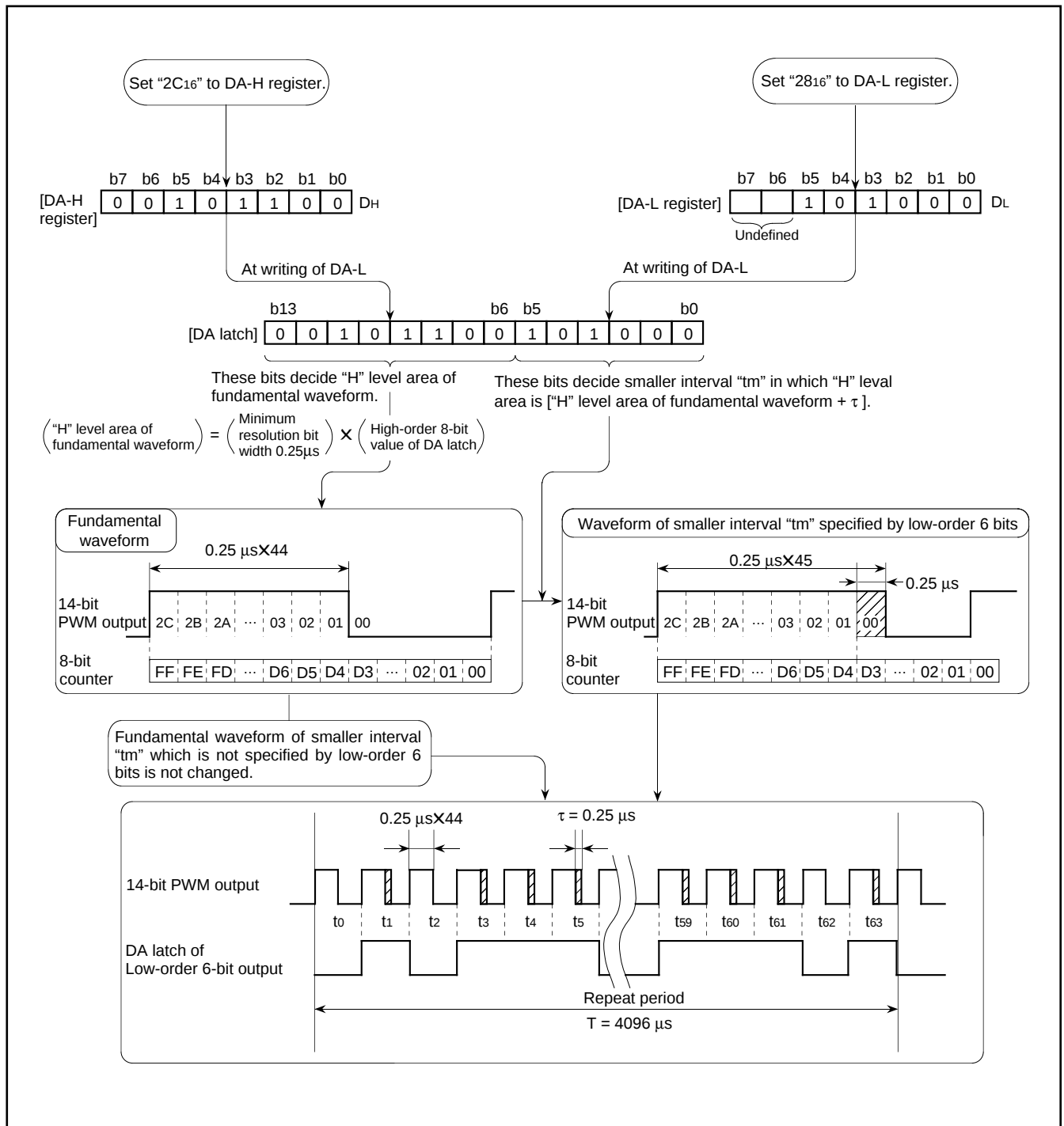
Fig. 15. 14-bit PWM output example ( f(X_{IN}) = 8 \text{ MHz} )
