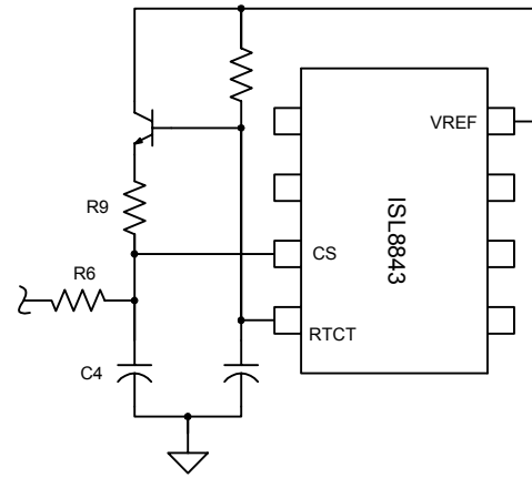
FIGURE 6. SLOPE COMPENSATION
