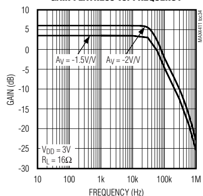
GAIN FLATNESS vs. FREQUENCY
