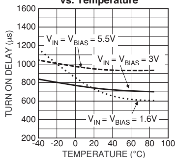
Turn On Delay vs. Temperature
