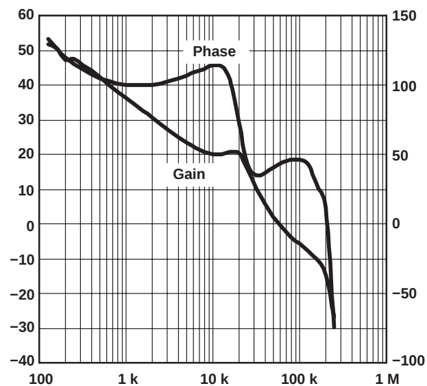
Figure 2–9. Measured Loop Response, TPS54610, V_{IN} = 3 \text{ V}
