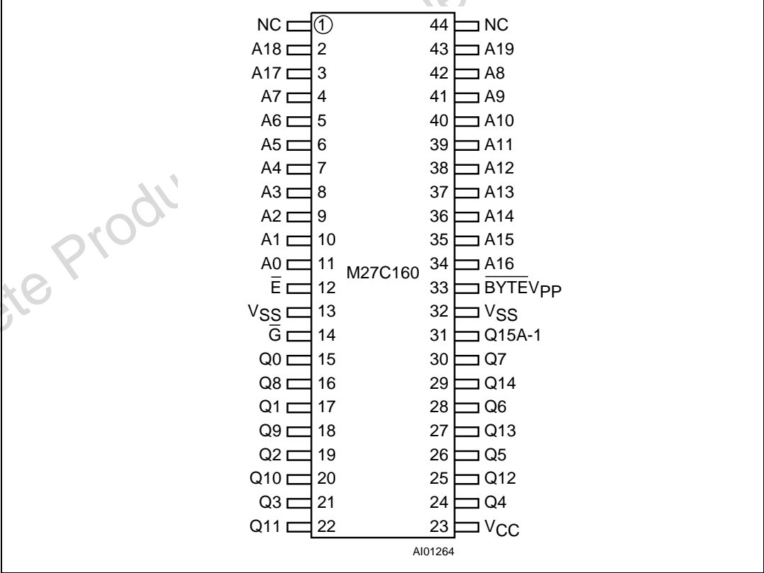
Figure 4. SO Connections
