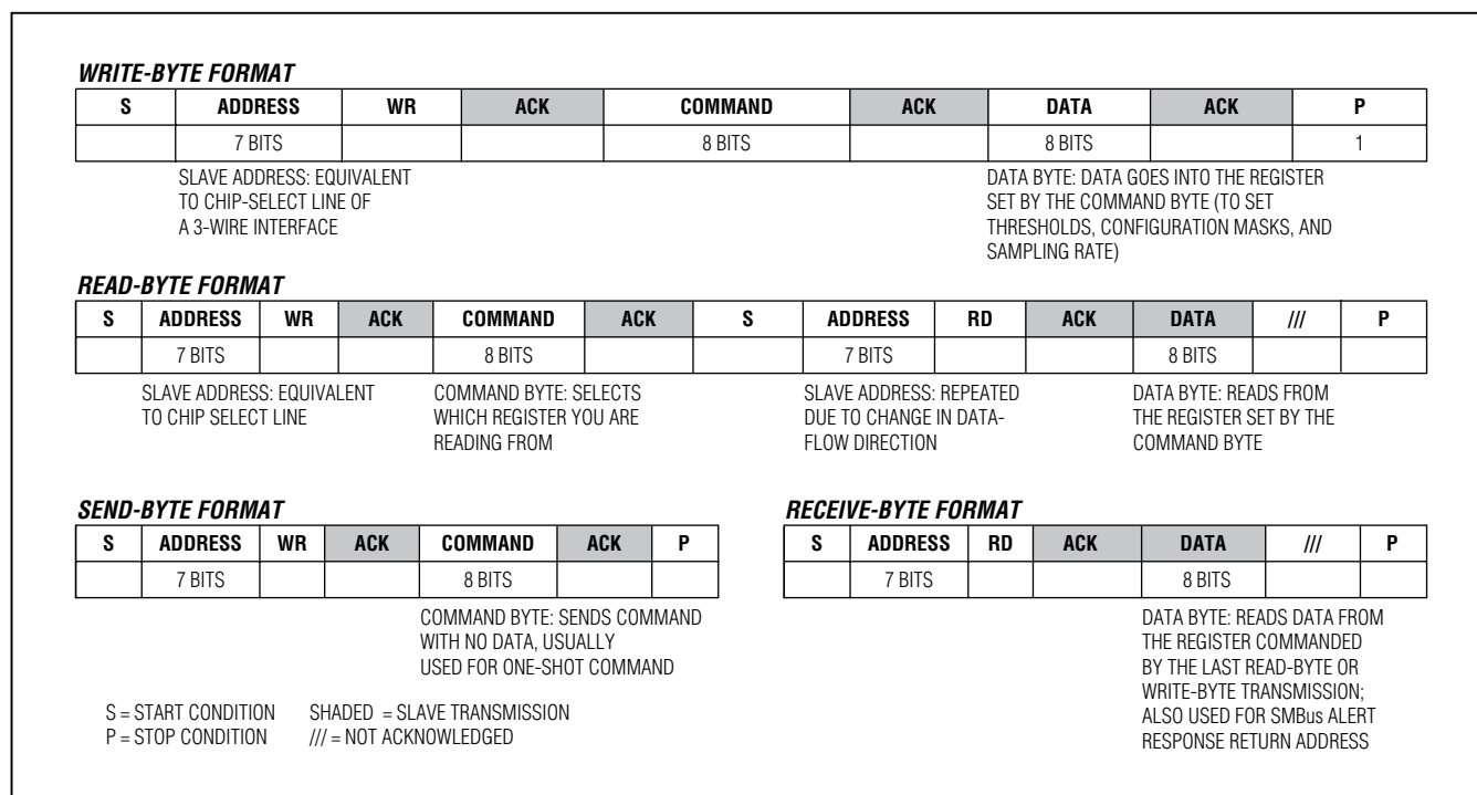
Figure 2. SMBus Protocols
