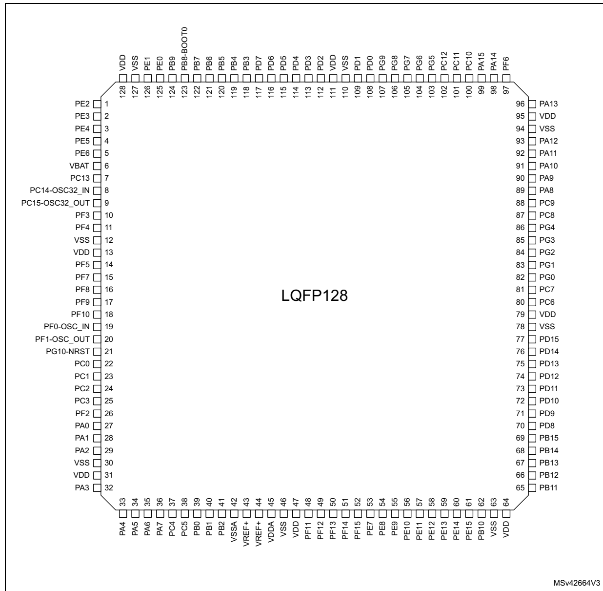
Figure 11. STM32G473xB/xC/xE LQFP128 pinout
