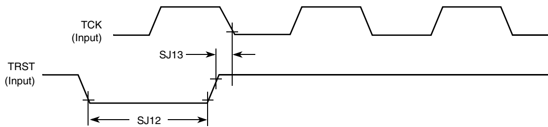
Figure 80. \overline{\text{TRST}} Timing Diagram
