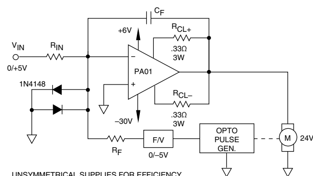
UNSYMMETRICAL SUPPLIES FOR EFFICIENCY
