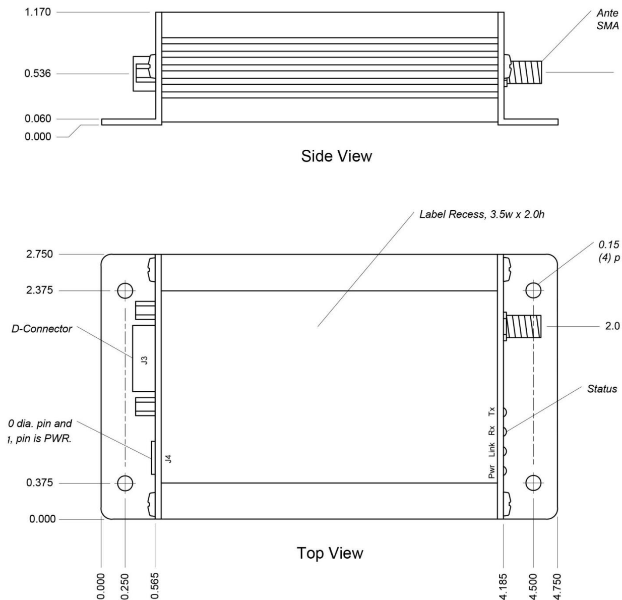
Figure 11: CL4490 Mechanical
