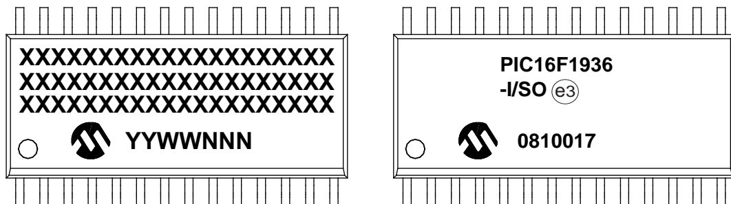
28-Lead SOIC (7.50 mm)
