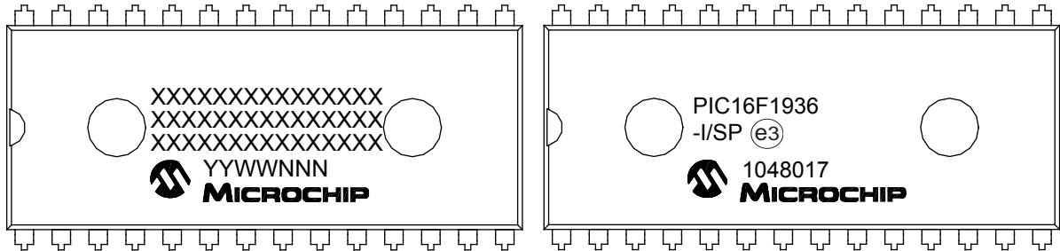
40-Lead PDIP (600 mil)
