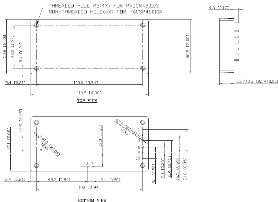
Mechanical Dimensions
