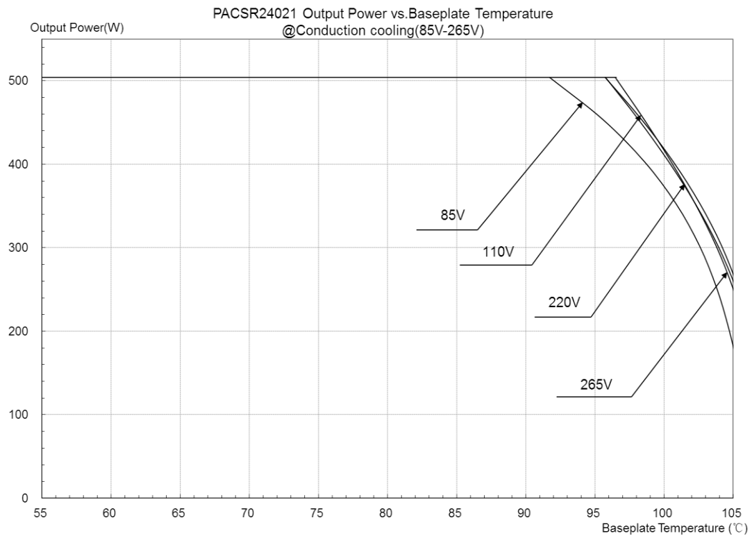
Figure 12: Thermal derating curves
