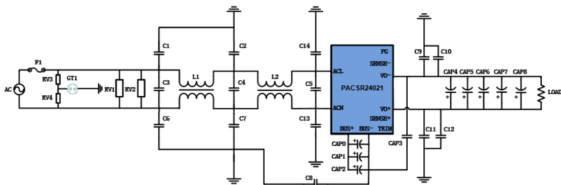
Figure 9: Application connection
