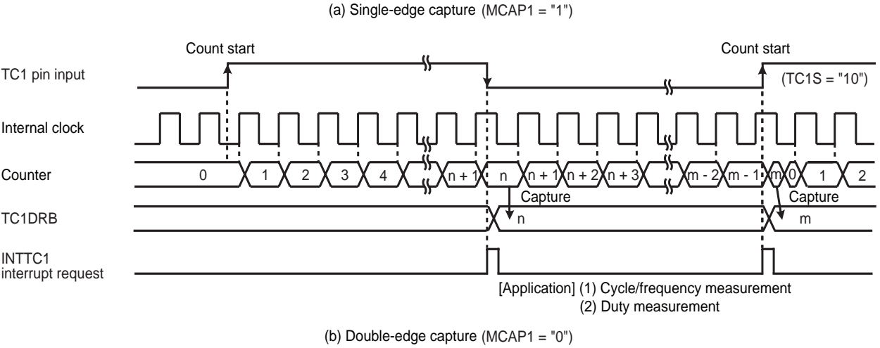
Figure 10-6 Pulse Width Measurement Mode
