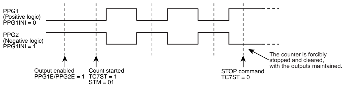
Figure 9-15 Immediately Stopping and Clearing the Counter with the Outputs Maintained (STM = 01)
