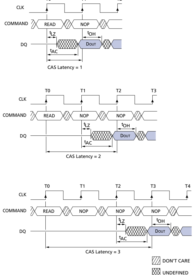
Figure 6 CAS Latency
