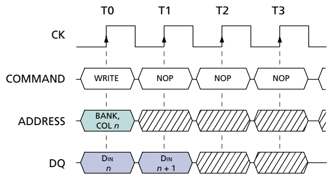
Figure 13 Write Burst
