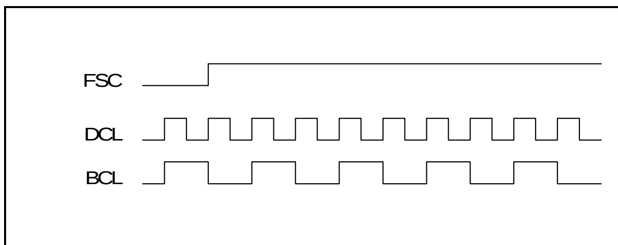
Figure 19 Clock waveforms
