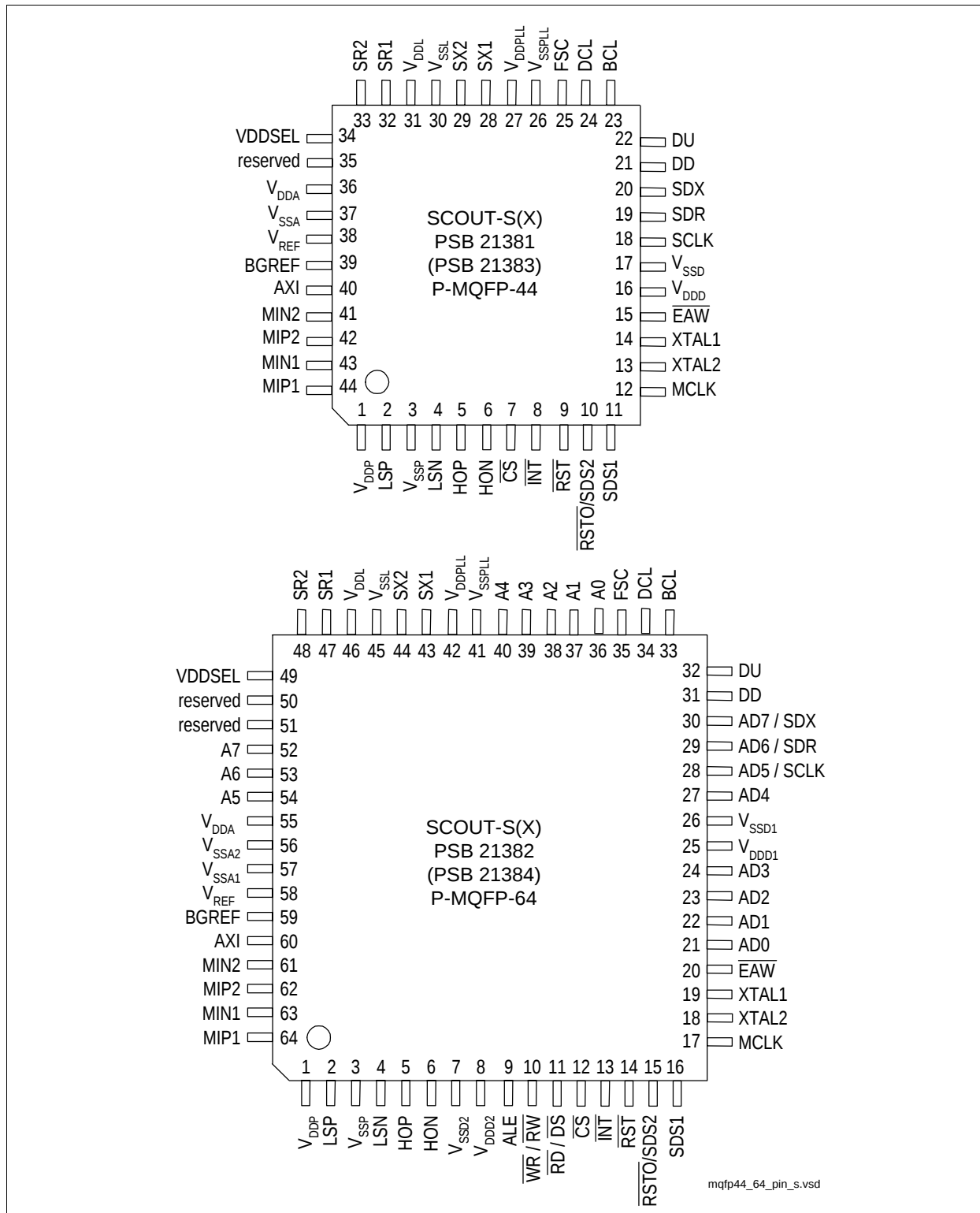
Figure 1 Pin Configuration
