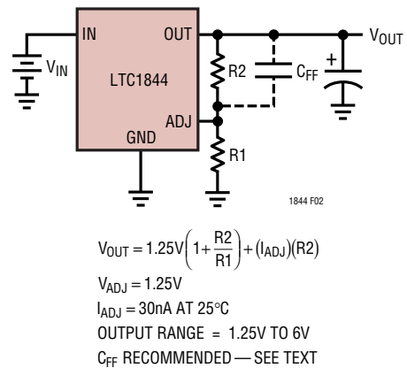
Figure 2. Adjustable Operation
