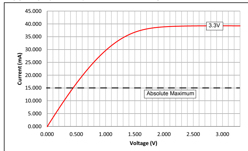
FIGURE 31-3: V_{OL} – 4x DRIVER PINS
