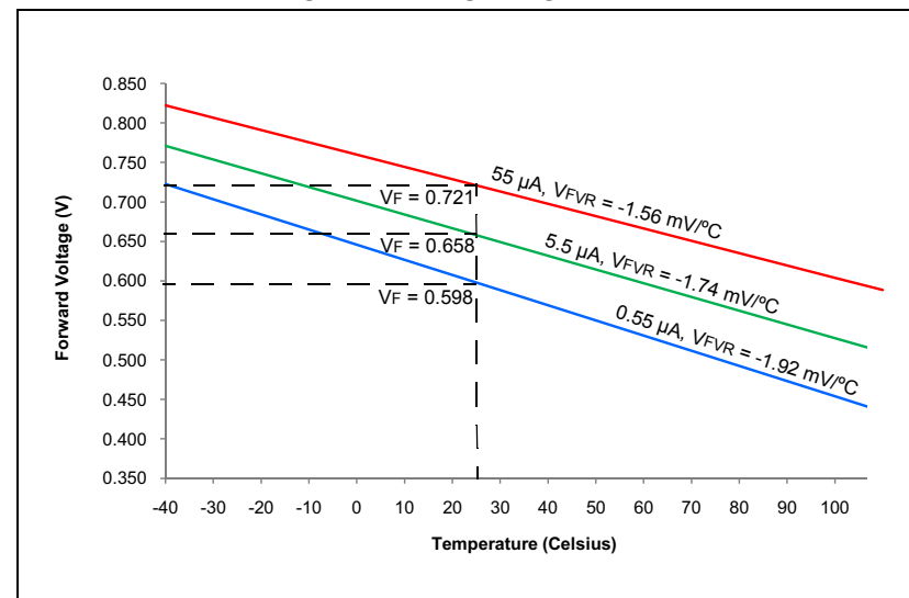
FIGURE 31-16: TYPICAL CTMU TEMPERATURE DIODE FORWARD VOLTAGE
