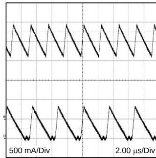
Figure 33. CCM and DCM Operating Modes V_{IN} = 24 \text{ V} , V_O = 3.3 \text{ V} , I_O = 2 \text{ A} /0.32 A 2 \mu\text{s/div}
