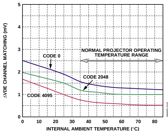
Figure 2. Channel Matching vs. Temperature
