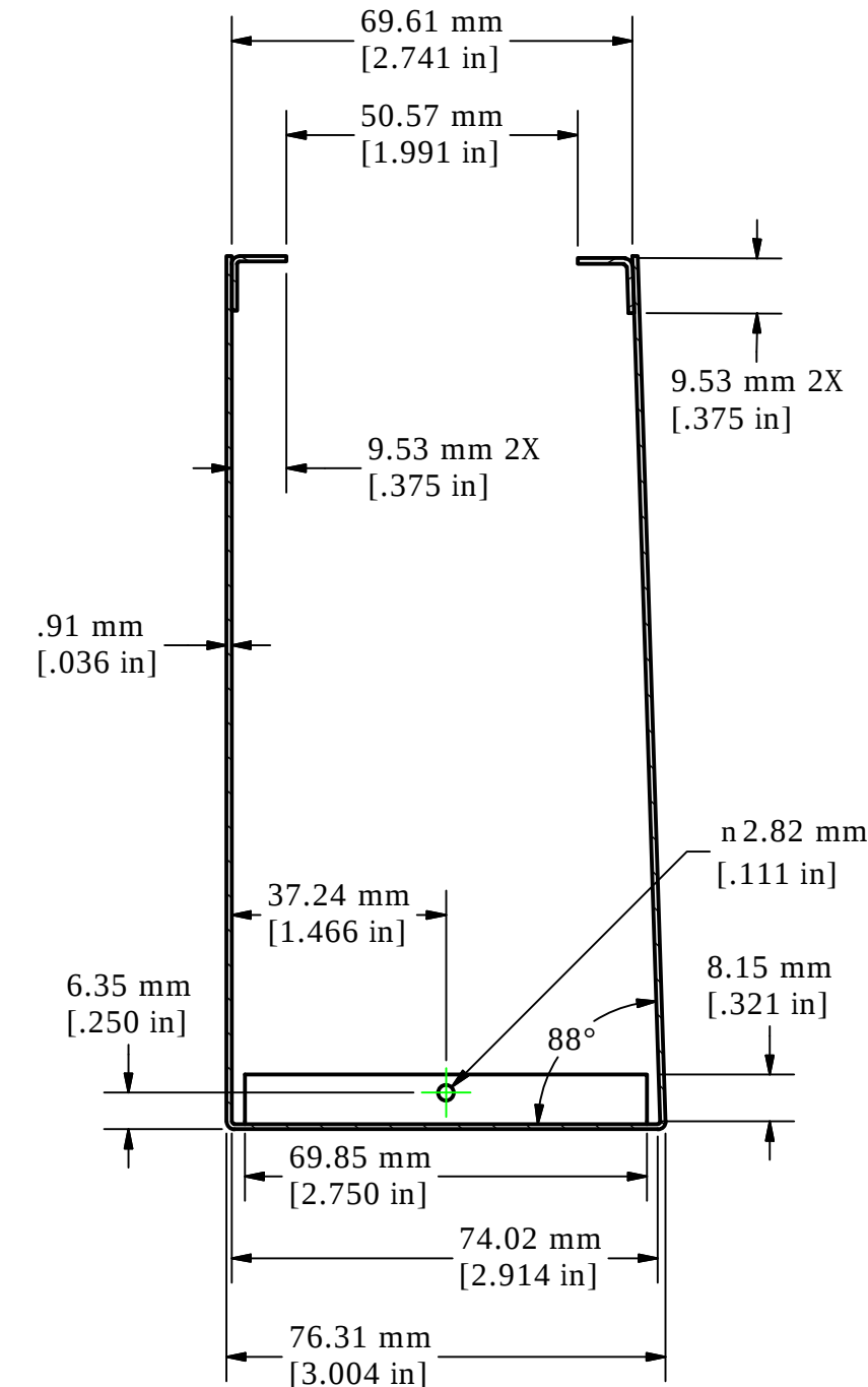
SECTION A-A SIDE SECTION VIEW OF EXPLODED ASSEMBLY
