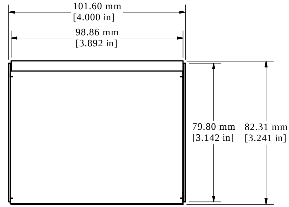
BOTTOM VIEW OF ASSEMBLY
