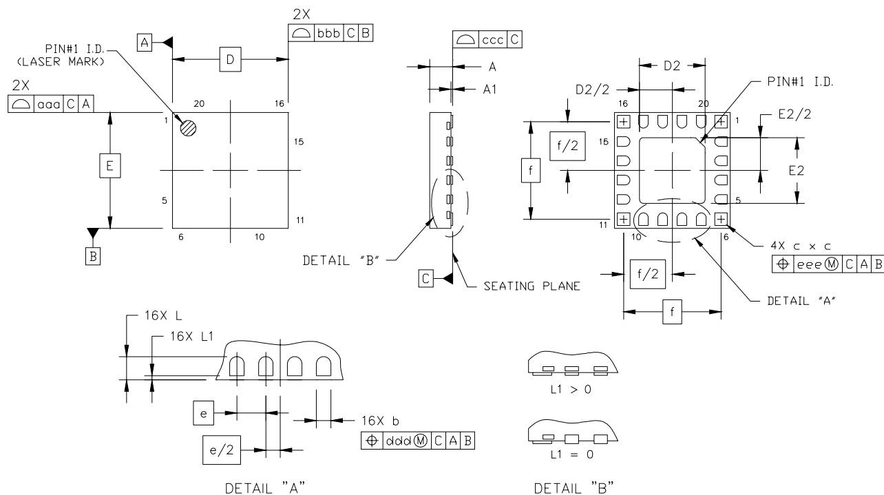
Figure 22. 20-Pin Quad Flat No-Lead (QFN)
