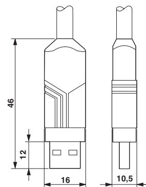
USB plug connector, type A, Standard
