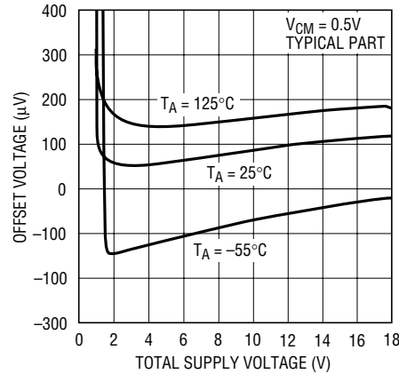
Input Offset Voltage vs Total Supply Voltage
