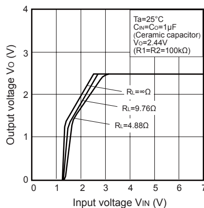
Fig.5 Output Voltage vs. Input Voltage (Typical Value)
