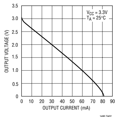
Driver Differential Output Voltage vs Output Current
