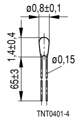
Dimensions in mm
