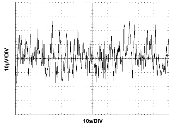
FIGURE 27. V_{OUT} NOISE
