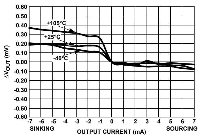
FIGURE 106. LOAD REGULATION
