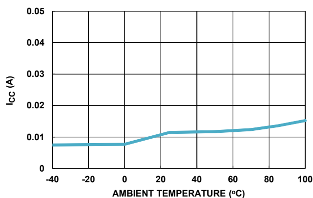
FIGURE 7. SHUTDOWN SUPPLY CURRENT vs TEMPERATURE
