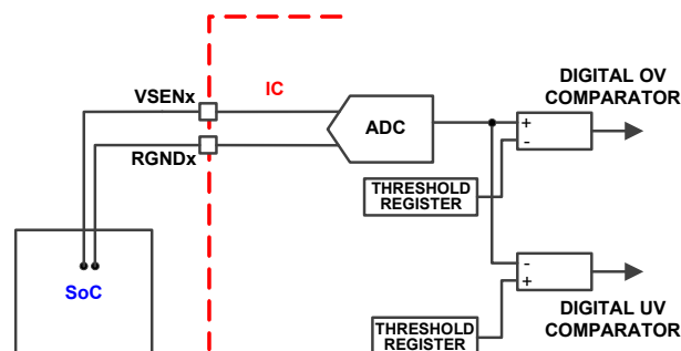
FIGURE 18. OVP, UVP COMPARATORS
