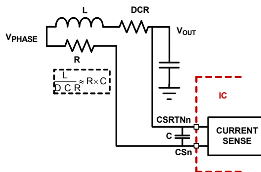
FIGURE 9. DCR SENSING CONFIGURATION
