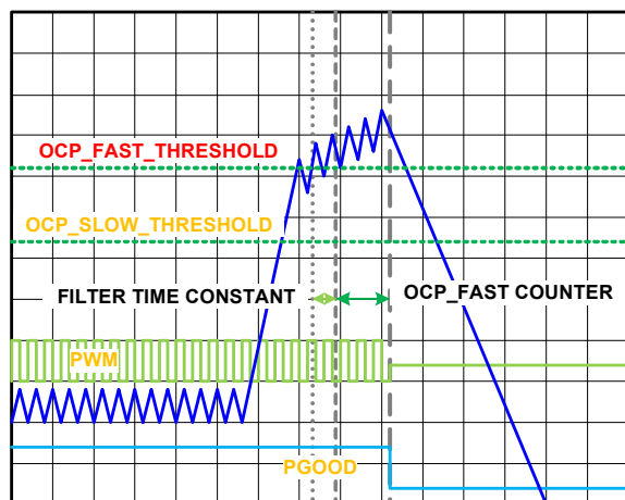
FIGURE 20. OCP_FAST
