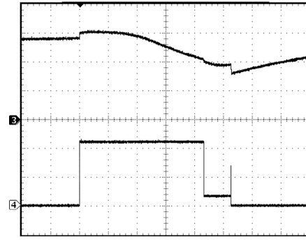
Time Base: 200 \mu s/div Circuit of Figure 43 Single LED I_{LED} = 1.2 A Ch 3: NTC pin voltage (5 V/div) Ch 4: I_{LED} (500 mA/div) R(T) = 100 k \Omega at 25°C R3 = 9 k \Omega
