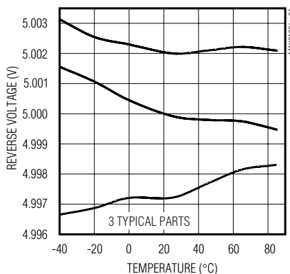
MAX6138_50 TEMPERATURE DRIFT
