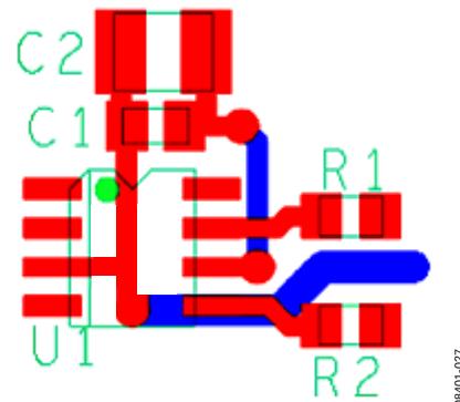
Figure 24. External Component Placement Example
