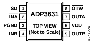
Figure 9. ADP3631 Pin Configuration
