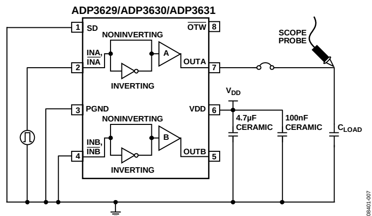
Figure 20. Test Circuit
