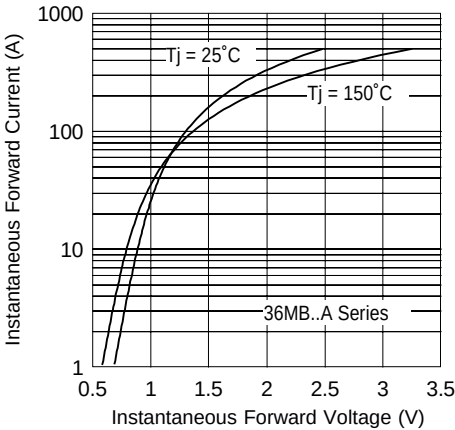
Fig. 7 - Forward Voltage Drop Characteristics Maximum Allowable Ambient Te
