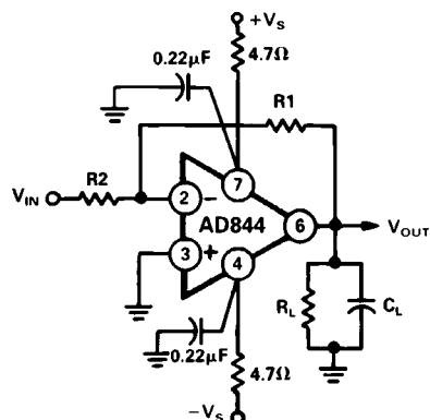
Figure 10. Inverting Amplifier, Gain of -1 ( R_1 = R_2 )
