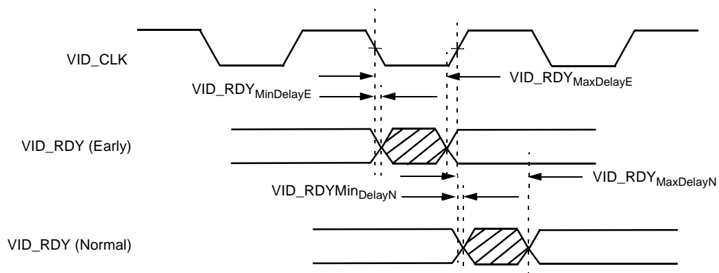
Figure 5-7. VID_RDY Delays
