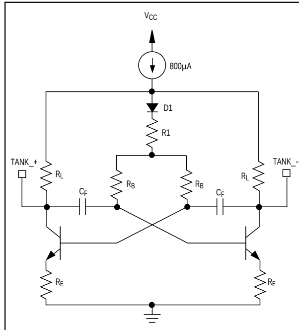
Figure 4. Voltage-Controlled Oscillators
