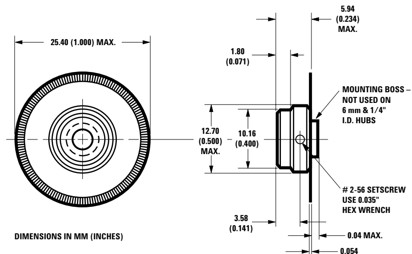
Figure 4. HEDS-5120 Codewheel.
