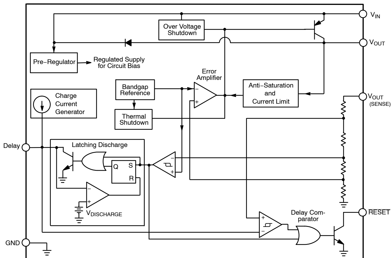
Figure 1. Block Diagram
