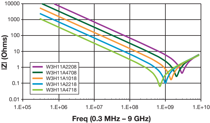
IMPEDANCE 0612 – 100V
