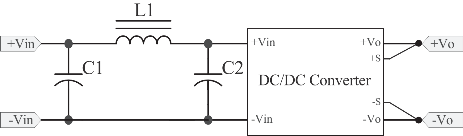
Figure 3 Recommended Circuit for EN55022 Class B (for all 3.3, 5, 12, 15, 24, & 28 Vdc output models)
