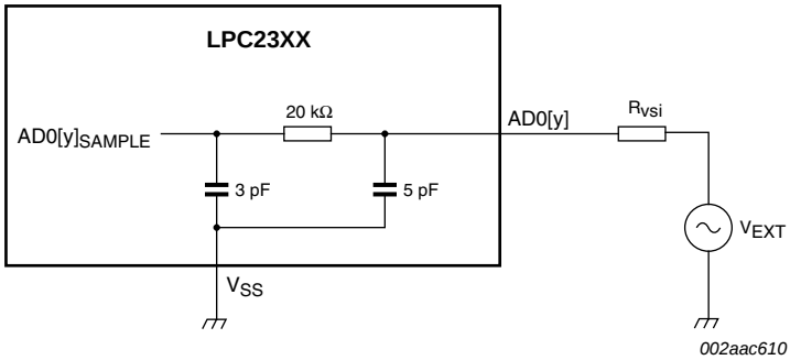
Fig 15. Suggested ADC interface - LPC2364/65/66/67/68 AD0[y] pin
