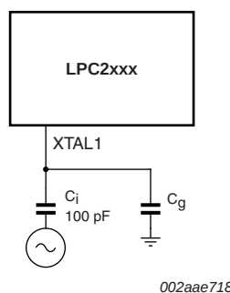
Fig 18. Slave mode operation of the on-chip oscillator
