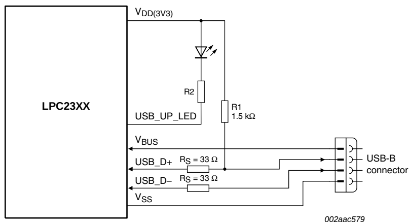
Fig 17. LPC2364/66/68 USB interface on a bus-powered device
