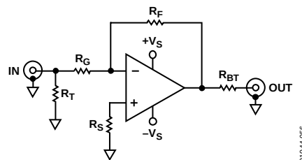
Figure 57. Inverting Configuration
