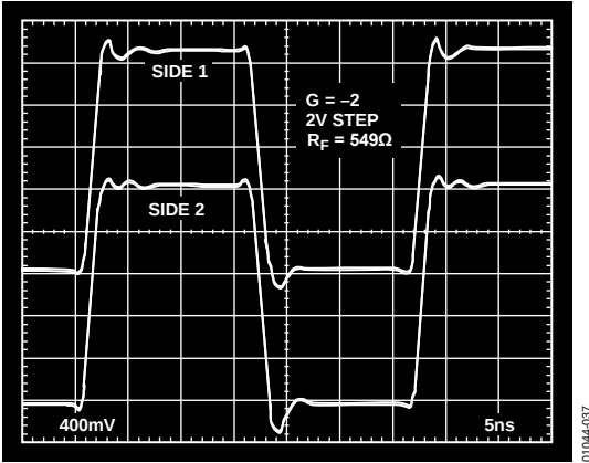
Figure 38. 2 V Step Response, G = -2
