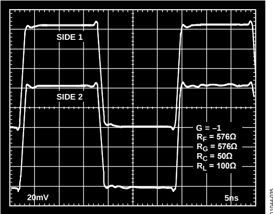
Figure 36. 100 mV Step Response, G = -1
