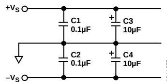
Figure 58. Supply Bypassing
