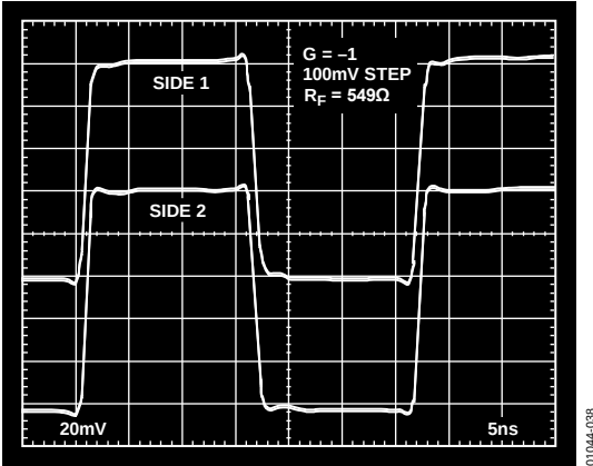
Figure 39. 100 mV Step Response, G = -1
