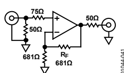
Figure 41. Frequency Response and Flatness Test Circuit (See Figure 10)
