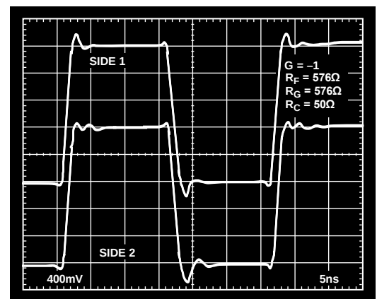
Figure 35. 2 V Step Response, G = -1
