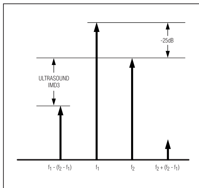
Figure 2. Ultrasound IMD3 Measurement Technique
