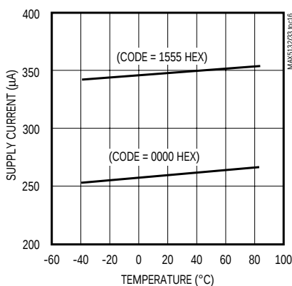
MAX5133 SUPPLY CURRENT vs. TEMPERATURE
