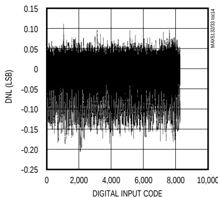
MAX5133 DIFFERENTIAL NONLINEARITY vs. DIGITAL INPUT CODE
