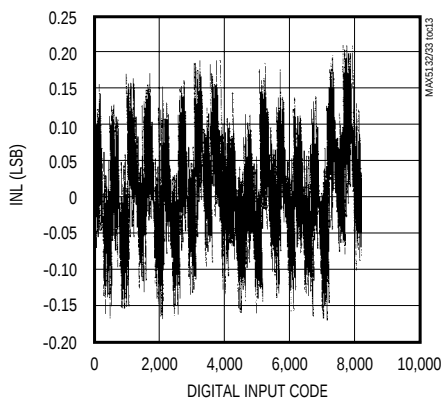
MAX5133 INTEGRAL NONLINEARITY vs. DIGITAL INPUT CODE
