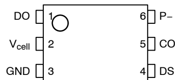
SON-6 (Top View)
