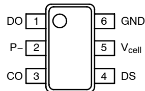
SOT23-6 (Top View)
