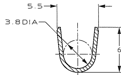
断面 "B" - "B" SECT "B" - "B"
