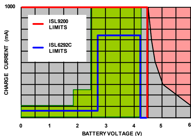
FIGURE 23. LITHIUM-SAFE OPERATING REGIONS
